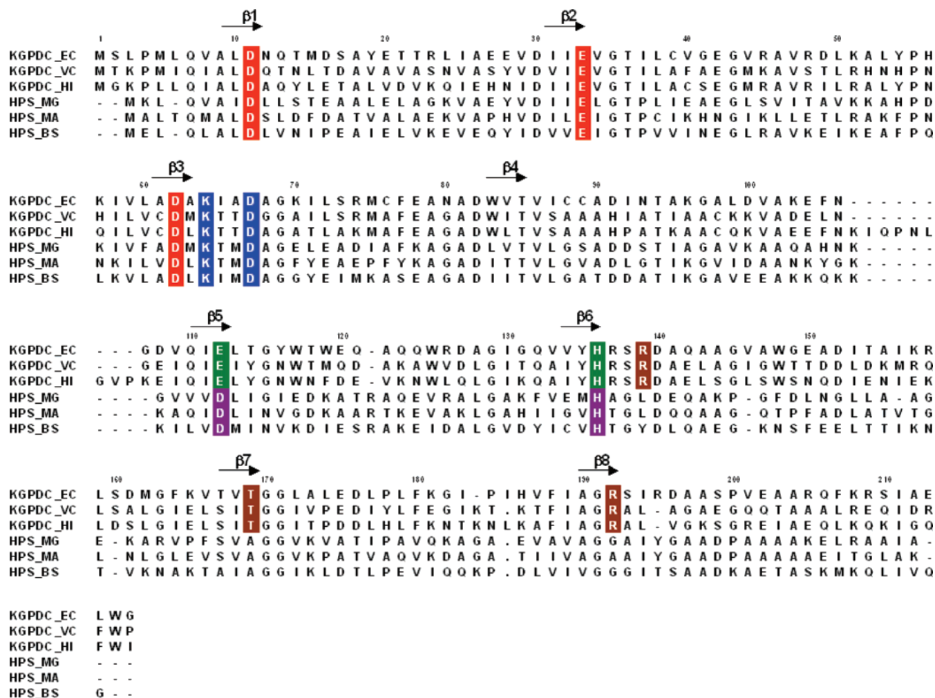
FIGURE 2: Sequence alignment of KGPDC's from E. coli (KGPDC_EC), Vibrio cholera (KGPDC_VC), and Haemophilus influenza (KGPDC_HI); and HPS's from Mycobacterium gastri (HPS_MG), M. aminofaciens (HPS_MA), and B. subtilis (HPS_BS). The strictly conserved Mg^{2+} ligands, Asp 11, Glu 33 and Asp 62, are highlighted in red. Lys 64 and Asp 67, residues involved in binding and stabilizing the cis -enediolate intermediate, are highlighted in blue. The His 136-Glu 112 dyads in the KGPDC's are highlighted in green, and the presumed His-Asp dyads in the HPS's are highlighted in magenta. In addition to Glu 112, the residues strictly conserved in KGPDC's that were targeted for mutagenesis, Arg 139, Thr 169, and Arg 192, are highlighted in brown. The alignment was produced by the Pileup algorithm of the GCG software package. Residues are numbered according to the KGPDC_EC sequence. The sequence identity between KGPDC's and HPS's is approximately 30%.
