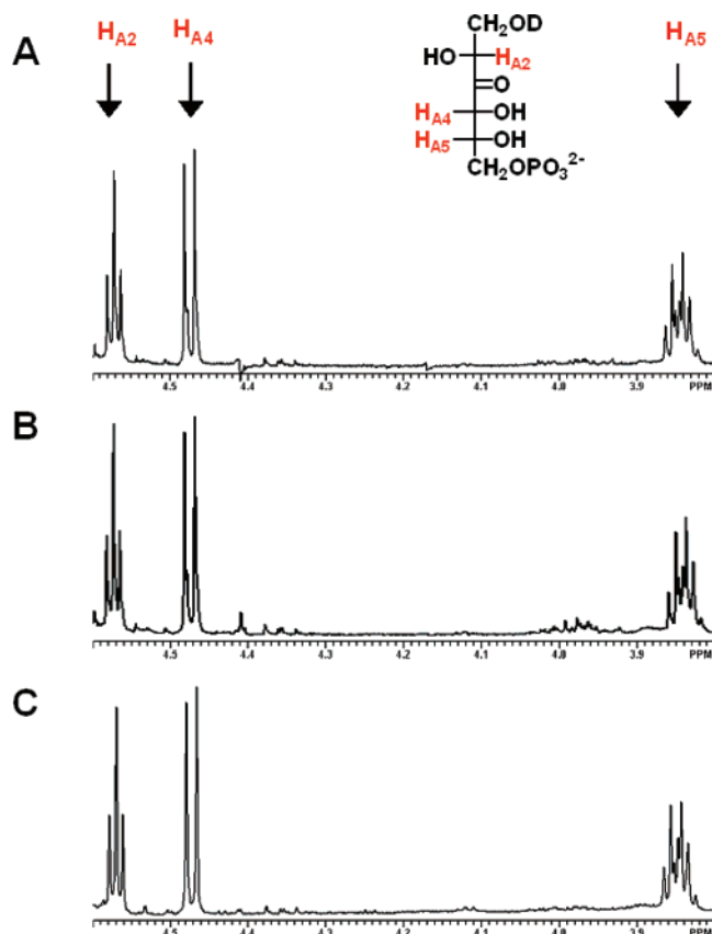
FIGURE 3: Partial ^1\text{H} NMR spectrum of D-arabino-hex-3-ulose 6-phosphate obtained from aldol condensation between D-ribulose 5-phosphate and formaldehyde in \text{D}_2\text{O} using (A) wild-type HPS, (B) wild-type KGPDC, and (C) the E112D/R139V/T169 mutant of KGPDC.
